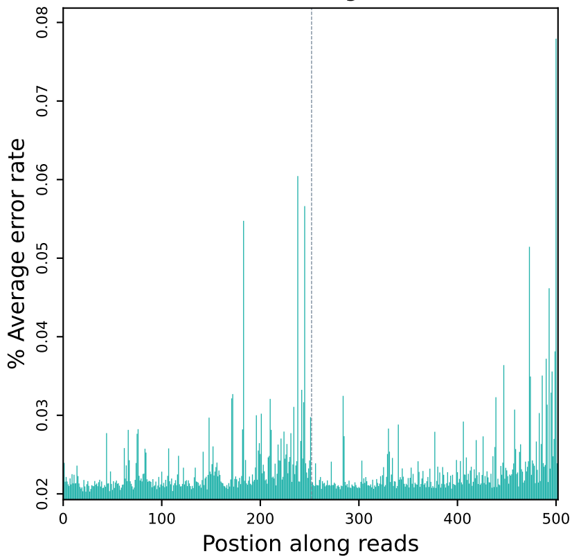
Error rate distribution along reads (R10525)
